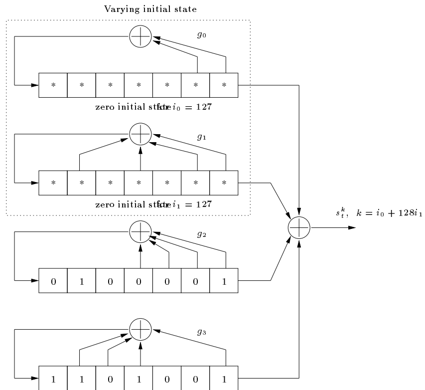
Figure 2: LFSR implementation of \mathcal{S}_o(2) for n = 7 with characteristic polynomials g_0(x) = x^7 + x + 1 , g_1(x) = x^7 + x^5 + x^3 + x + 1 , g_2(x) = x^7 + x^3 + x^2 + x + 1 , and g_3(x) = x^7 + x^5 + x^4 + x^3 + 1 .
