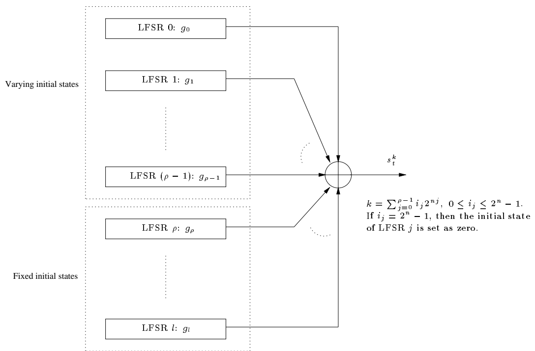
Figure 1: LFSR implementation of \mathcal{S}_o(\rho)
